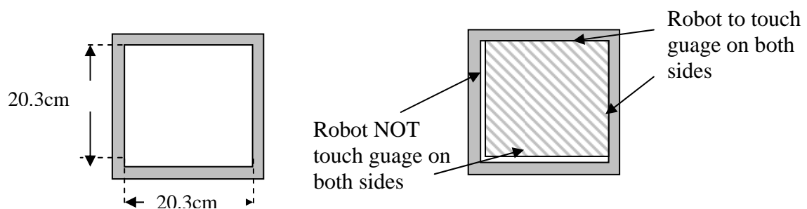
Figure 2: Caging Gauge
