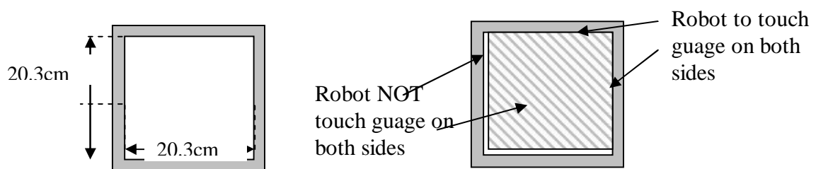
Figure 2: Caging Gauge
