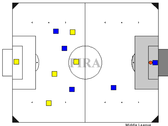
Figure 6 : Goal-Kick
