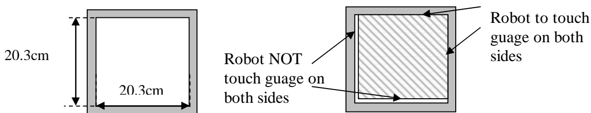
Figure 2: Caging Gauge
