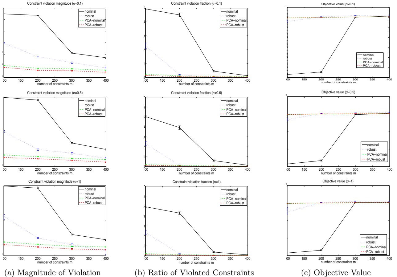
Figure 1: Performance comparison of nominal method (black), robust method (blue), PCA-nominal (green), and PCA-robust (red). We fix the dimensionality p = 100 , and vary the number of constraints m from 100 to 400. Three performance criteria are compared: (a) the magnitude of violation; (b) the fraction of violated constraints; and (c) the objective value. The first, second and third rows are for \sigma = 0.1 , \sigma = 0.5 and \sigma = 1 , respectively.
