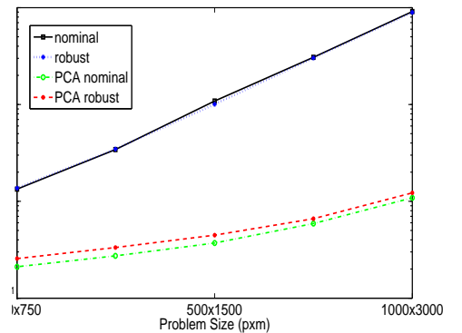
Figure 2: Computation time for different approaches.
